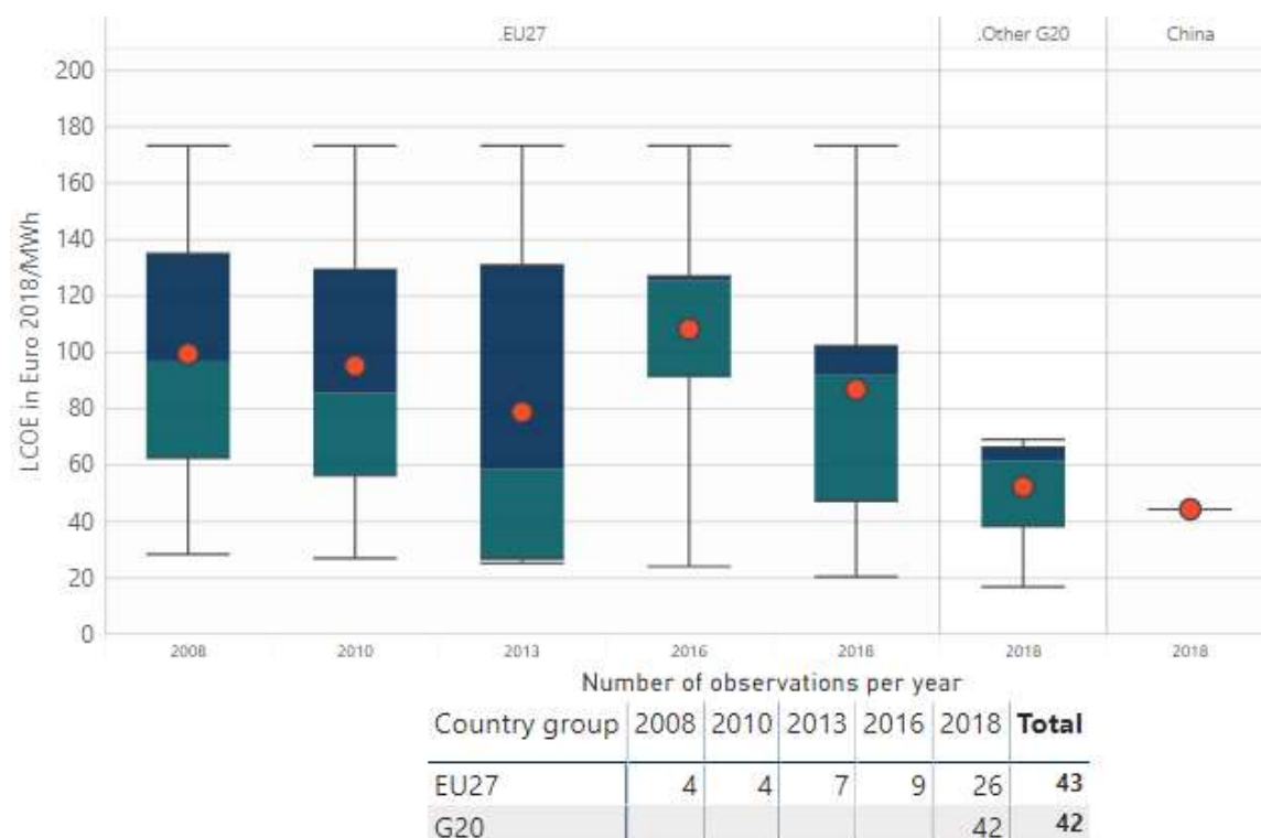
Figure 1-36 LCOH results for EU27 and G20 - Domestic solar thermal
