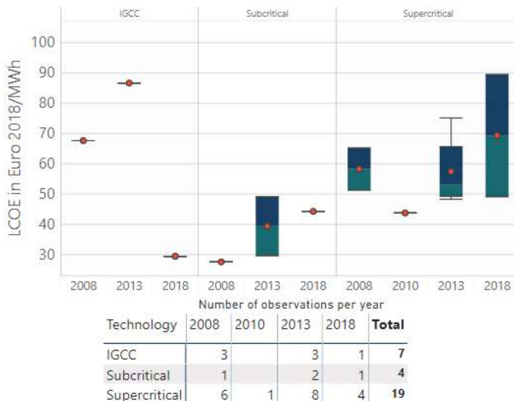
Figure 1-31 LCOE results for G20 - Coal (IGCC and Subcritical vs Supercritical)
