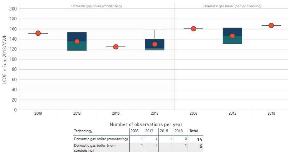
Figure 1-39 LCOH results for EU27 - Domestic gas boilers
