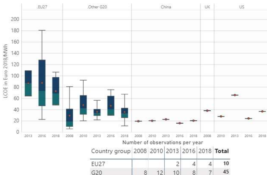
Figure 1-21 LCOE results for EU27 and G20 - Hydropower (inputs from IRENA)
