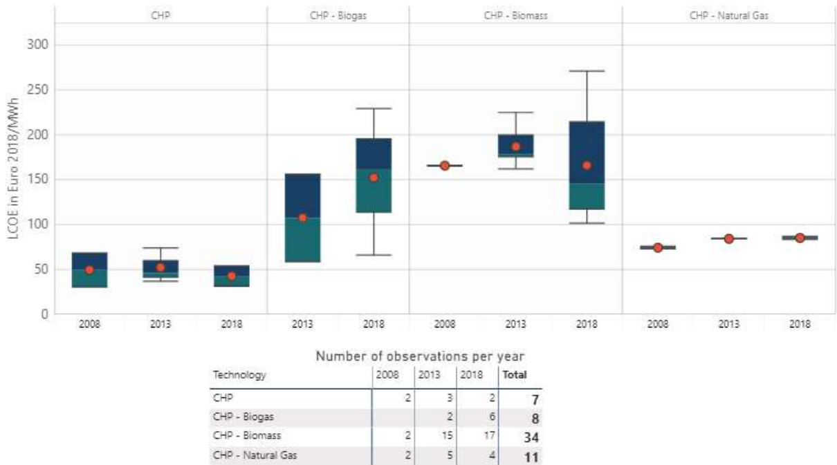
Figure 1-34 LCOE&LCOH results for EU27 - CHP (Natural gas, biofuels and undetermined fuels)
