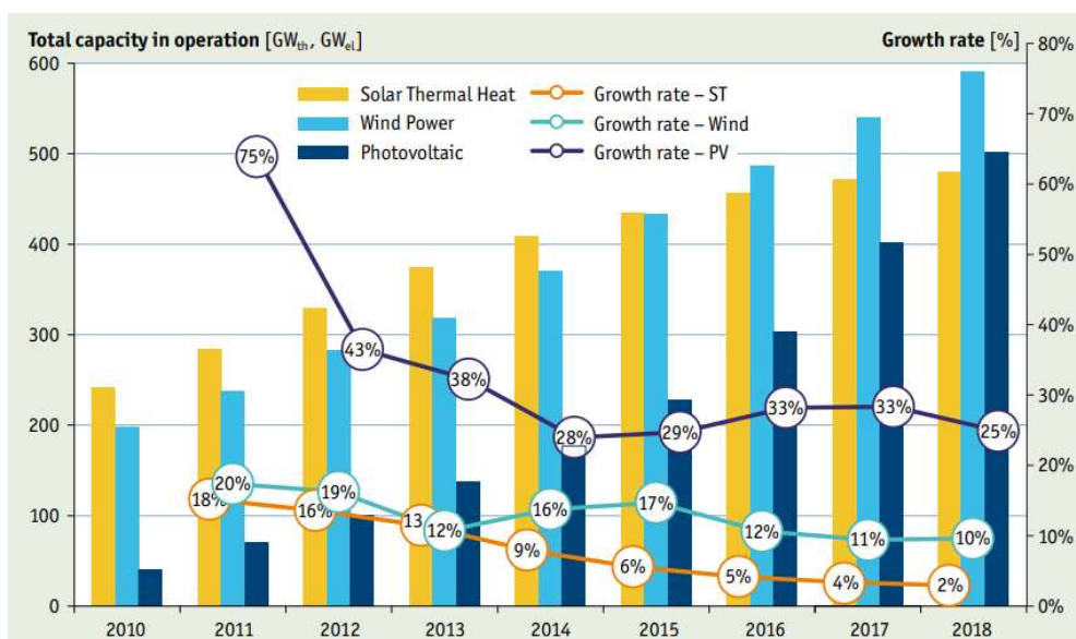
Figure 1-35 World installed capacity and growth of solar thermal and other RES
