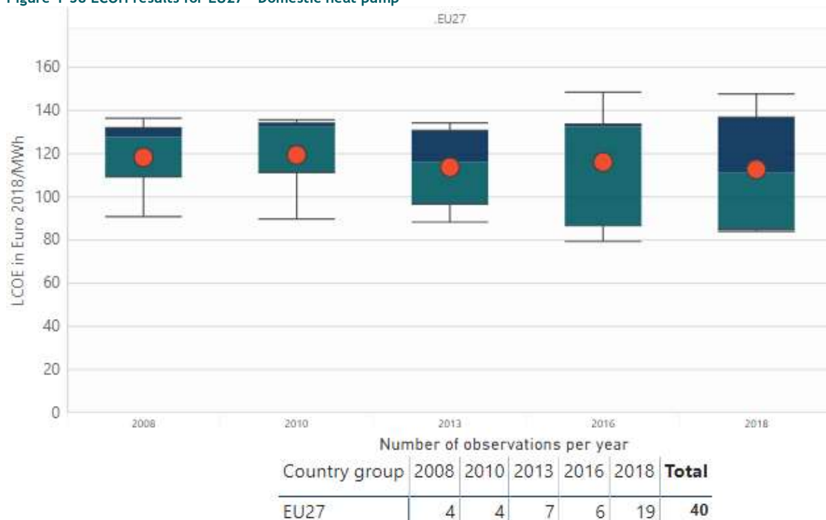
Figure 1-38 LCOH results for EU27 - Domestic heat pump
