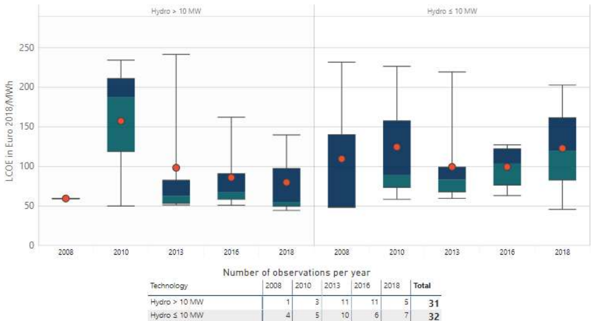
Figure 1-19 LCOE results for EU27 - Hydropower > 10 MW and Hydropower ≤ 10 MW
