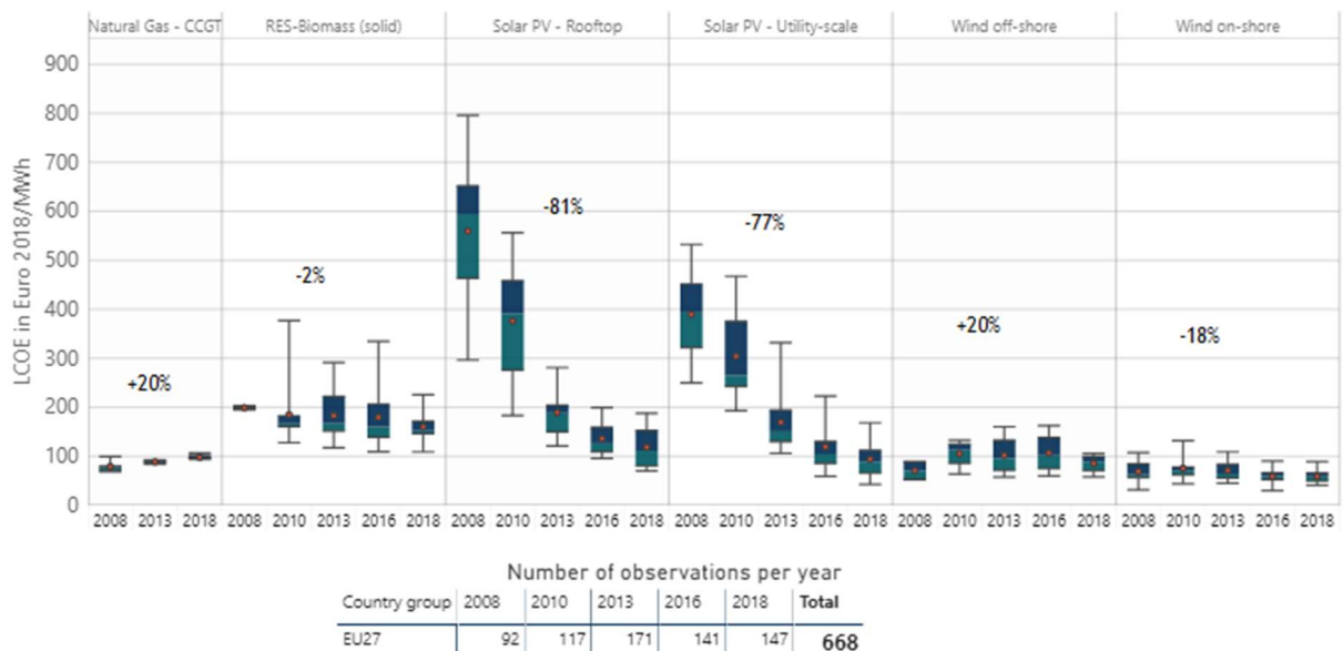
Figure 1-40 LCOE results for EU27 - main technologies comparison
