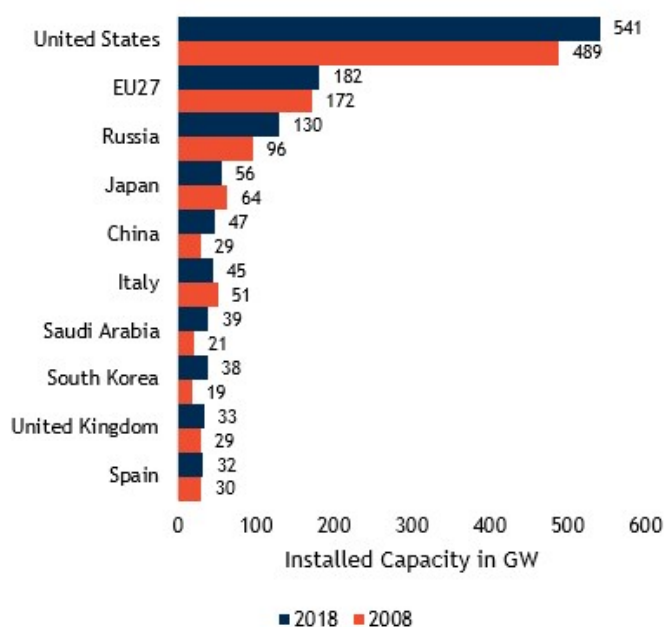
Figure 1-25 Installed Capacity in 2018 - Gas-fired installed capacity (GW)
