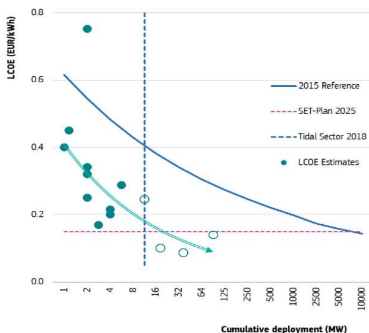
Figure 1-24 LCOE estimates for marine energy technologies
