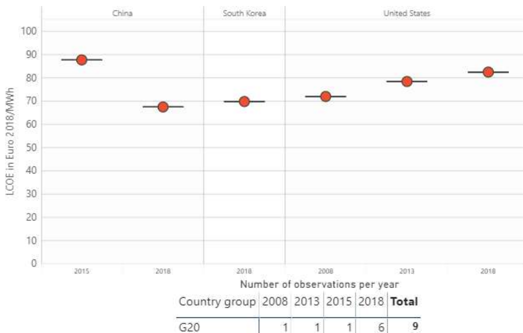
Figure 1-32 LCOE results for G20 - Nuclear
