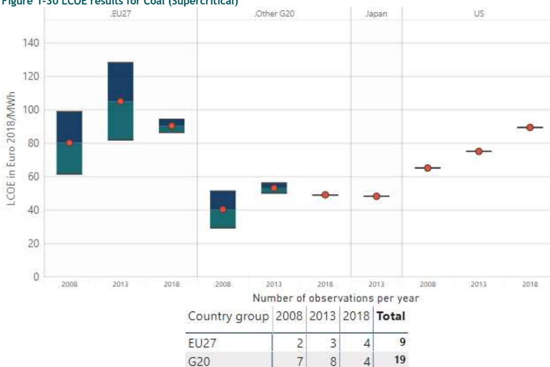
Figure 1-30 LCOE results for Coal (Supercritical)
