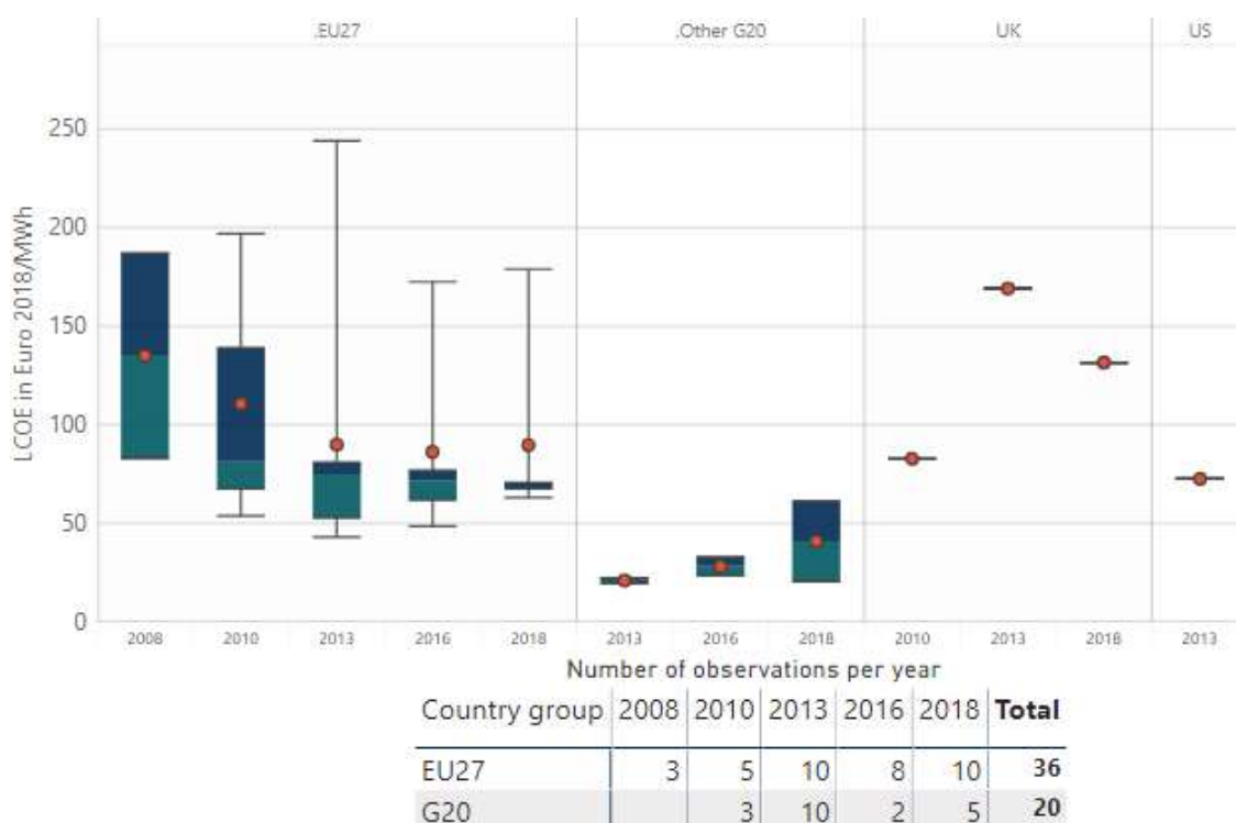
Figure 1-23 LCOE results for EU27 and G20 - Biogas
