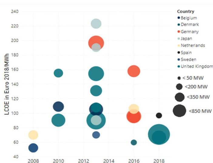
Figure 1-10 LCOE results for Wind off-shore projects by Installed Capacity
