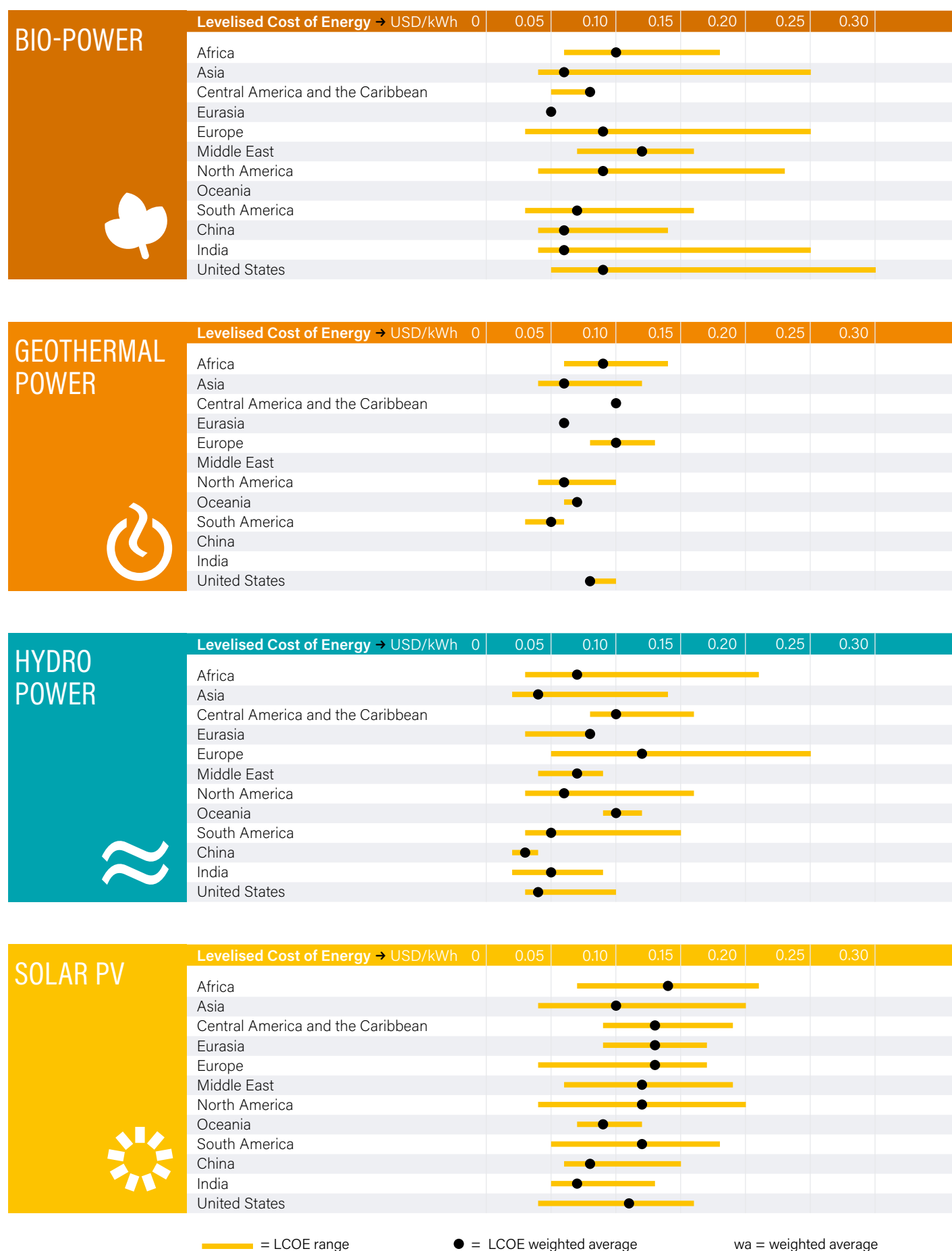
■ TABLE 3. Status of Renewable Electricity Generating Technologies, Costs and Capacity Factors, 2017
